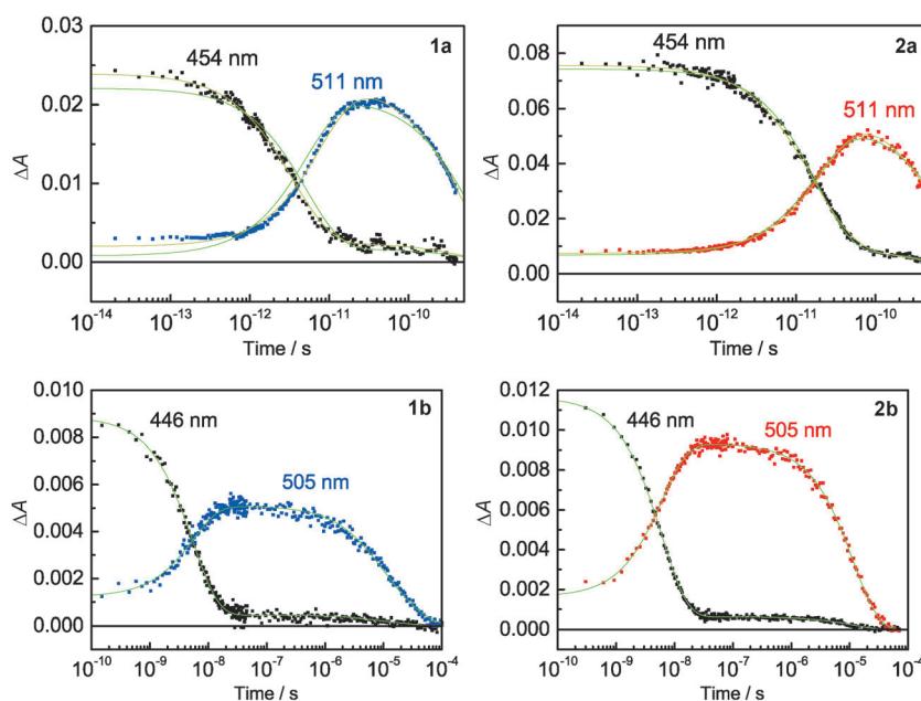
Figure 4. Transient absorption decay profiles of the derivatives in \text{CH}_2\text{Cl}_2 . Green and yellow curves represent the theoretical best fits to Equations (S7) and (S17), respectively.
