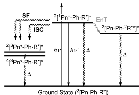
Figure 2. Excited-state processes of the pentacene–radical derivatives. Pn, Ph, and R' denote the pentacene, phenyl, and radical moieties, respectively.
